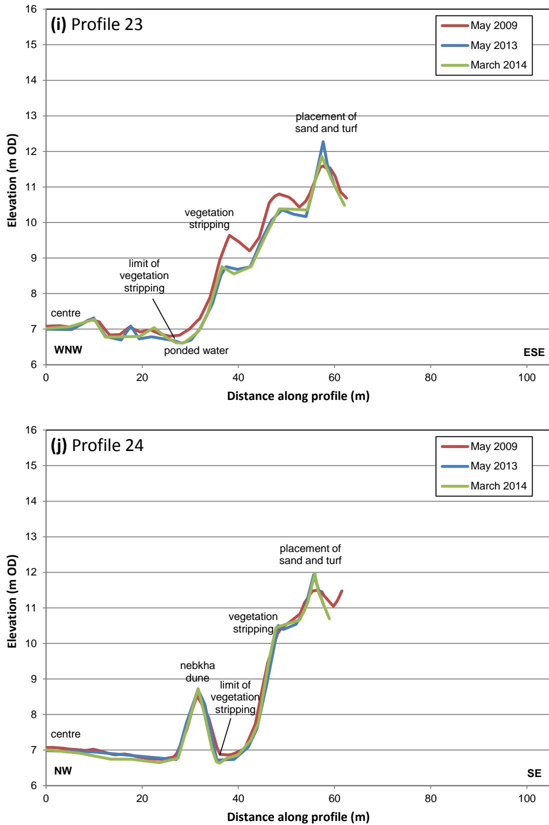
Figure 10. continued. Comparison of surface levels at profiles 23 and 24 in Area 3, indicated by LiDAR survey on 12th May 2009 (pre-works) and ground surveys on 17 May 2013 and 13 March 2014
